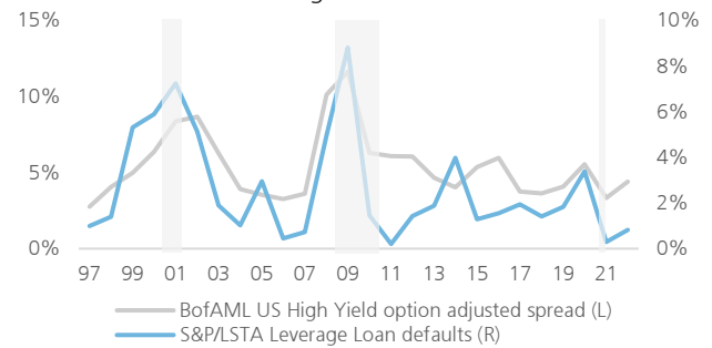
Fig. 4: High yield spreads and leveraged loan default rates
