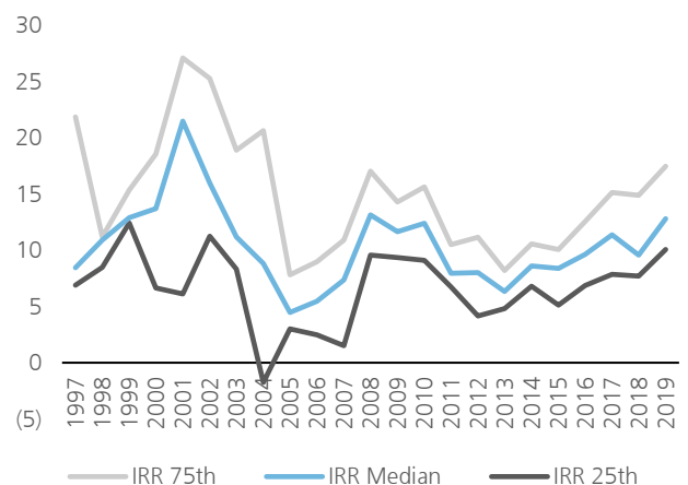
Fig. 3: Distressed debt IRR per vintage year 1997-2019
