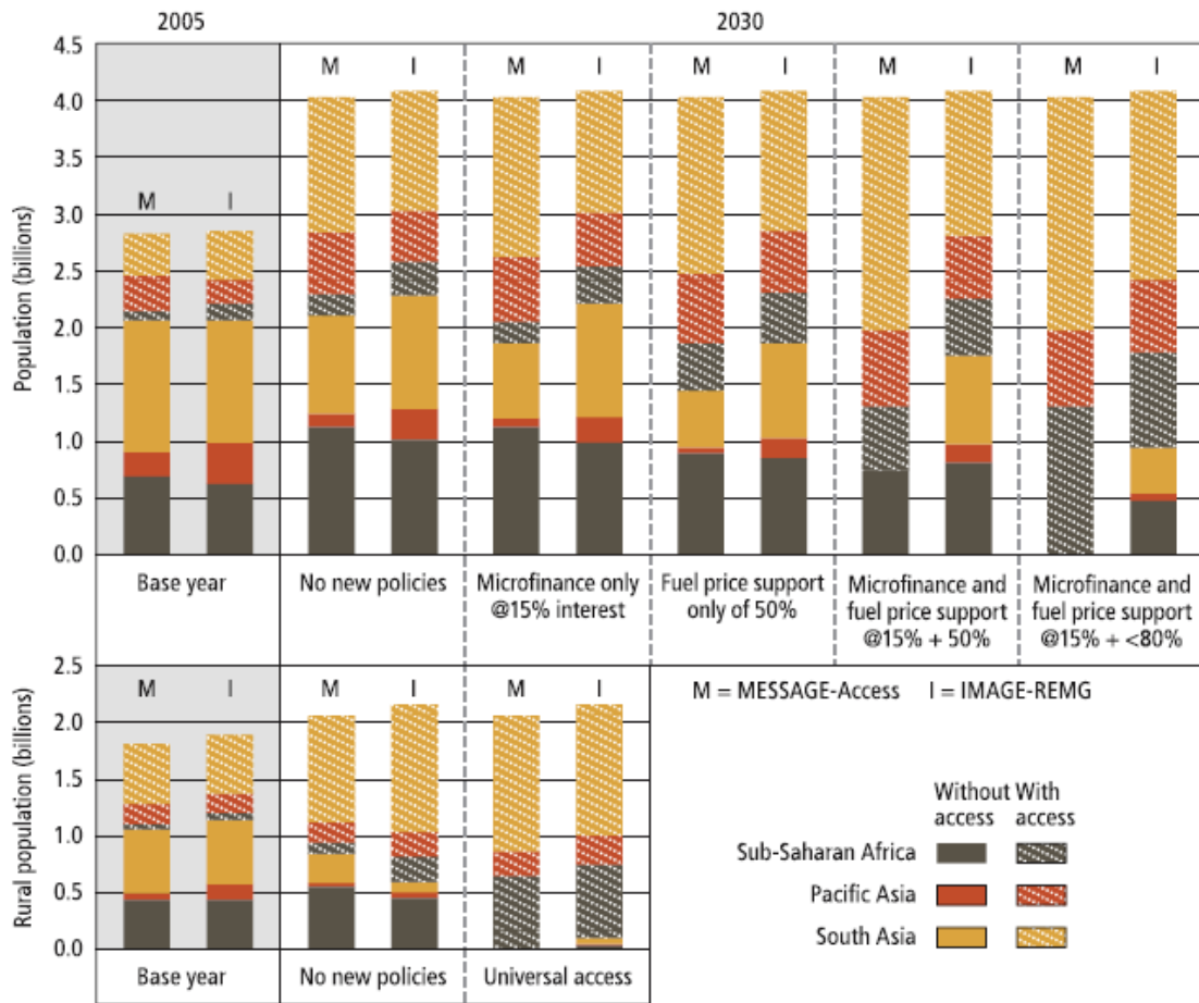
Figure 1. Impact of policies and price support on access to modern energy services and rural electrification under different policy scenarios
